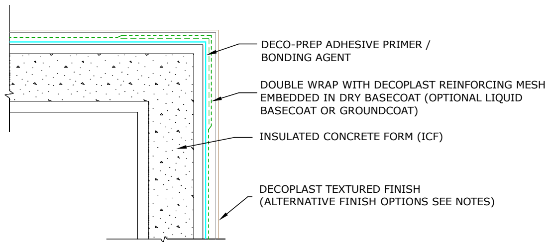
OUTSIDE CORNER
