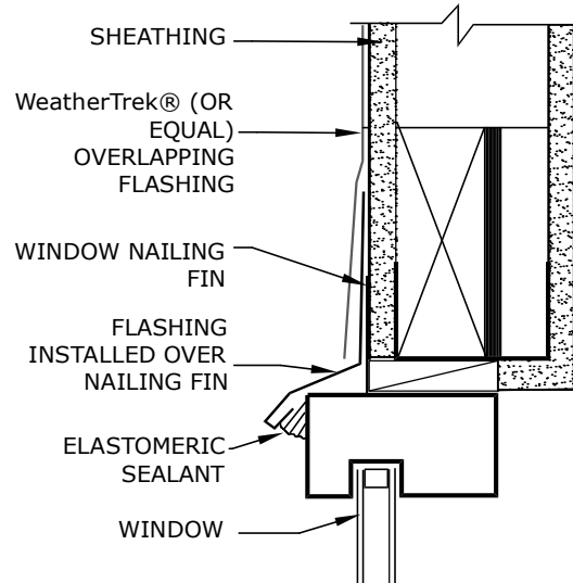
SECTION B-B WINDOW WITH NAILING FIN
