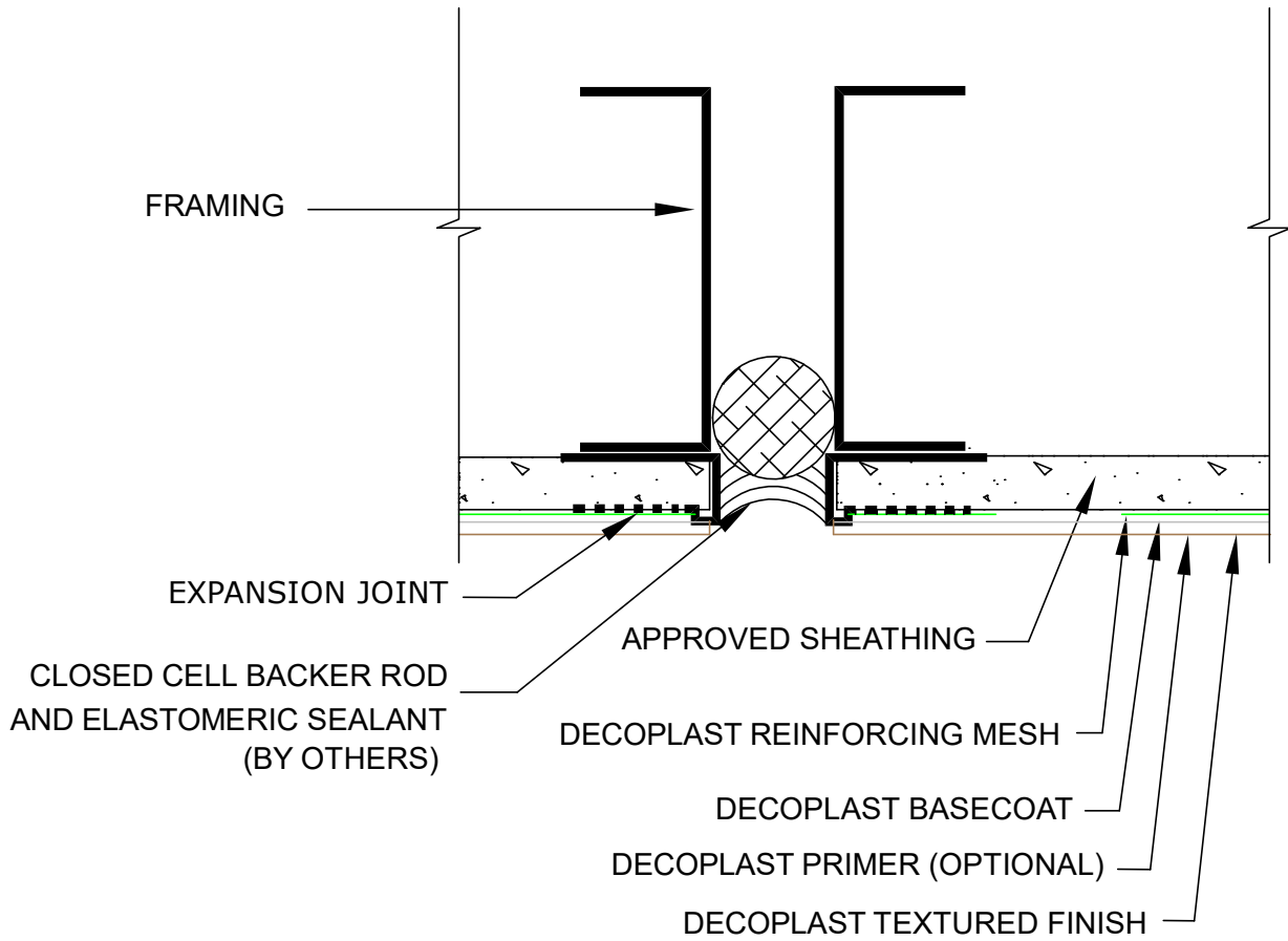
DACF SOFFIT 1.06 EXPANSION JOINT DETAIL
